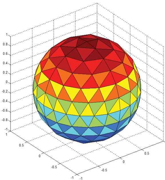
Fig. 7 Octahedral triangulation with n=6
